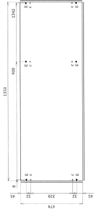
4. Capac Ios x 1buc. ( 1350 x 474 x 16 )
