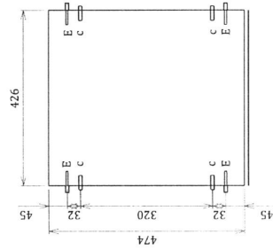
6. Polita Mica x 2buc. ( 426 x 474 x 16 )
