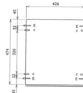
7. Polita Dulap x 2buc. ( 426 x 474 x 16 )
